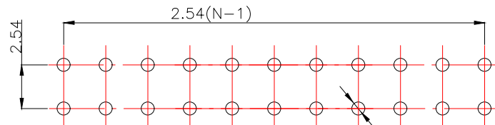
[P.C.B.LAYOUT]
