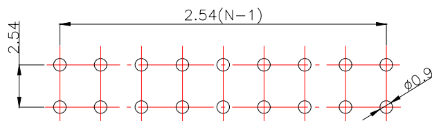
[P.C.B.LAYOUT]
