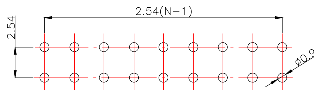
[P.C.B.LAYOUT]
