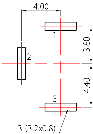
P.C.B LAYOUT(copper-side view)
