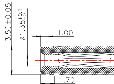
MATING PLUG
