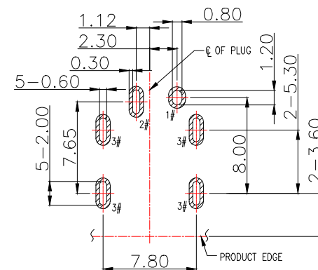
PCB.WELDING DRAWING (TOLERANCE:±0.05)
