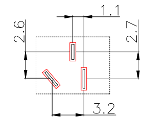
PCB.WELDING DRAWING (TOLERANCE:±0.05)
