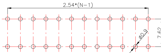
[P.C.B.LAYOUT]
