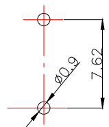
[P.C.B.LAYOUT]
