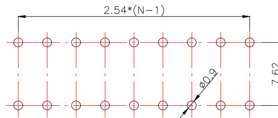
[P.C.B.LAYOUT]
