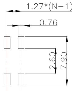
[P.C.B.LAYOUT]
