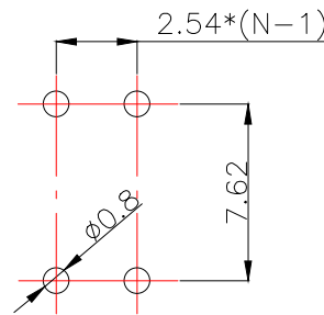
[P.C.B.LAYOUT]
