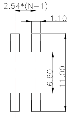
[P.C.B.LAYOUT]
