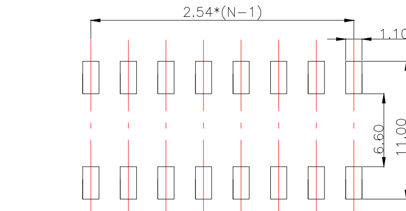
[P.C.B.LAYOUT]
