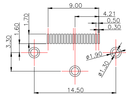
PCB LAYOUT(TOP VIEW) (T=1.60mm)
