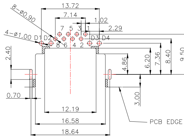
RECOMMENDED PCB LAYOUT (t=1.6mm,tol:±0.05)
