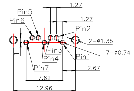
RECOMMENDED P.C.B. LAYOUT(TOP VIEW) THICKNESS:1.6mm; TOLERANCE ±0.05mm
