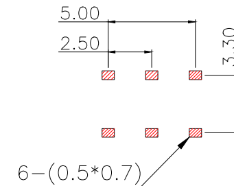
PCB.WELDING DRAWING (TOLERANCE:±0.05)
