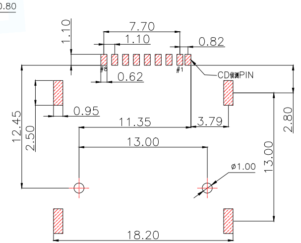
Recommended PCB Layout General tolerance \pm 0.05 weld zone
