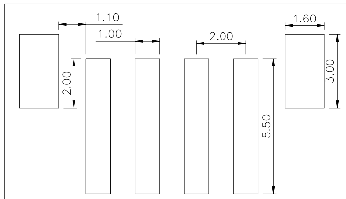
RECOMMENDED P.C.B HOLE LAYOUT
