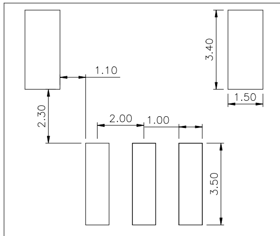
RECOMMENDED P.C.B HOLE LAYOUT
