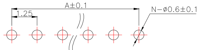
PCB.WELDING DRAWING
