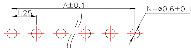
PCB.WELDING DRAWING
