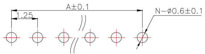
PCB.WELDING DRAWING
