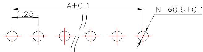
PCB.WELDING DRAWING
