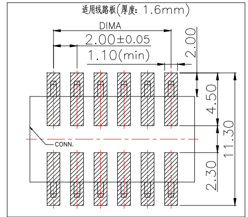
PCB.WELDING DRAWING (TOLERANCE:±0.05)
