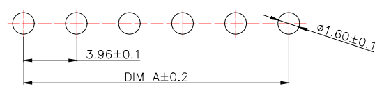
SUGGESTED PCB LAYOUT (COMPONENT SIDE)
