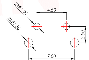
PCB.WELDING DRAWING
