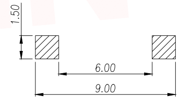
PCB.WELDING DRAWING
