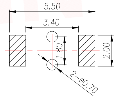
PCB.WELDING DRAWING
