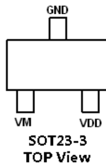
Figure 2. PIN Configuration
