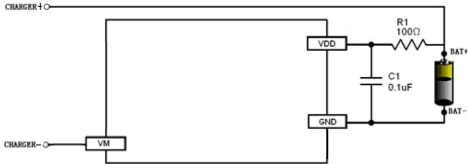
Fig 6 XB3153IS in a Typical Battery Protection Circuit
