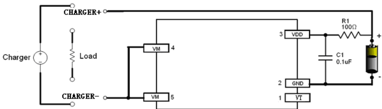
Fig 6 XB5350A in a Typical Battery Protection Circuit
