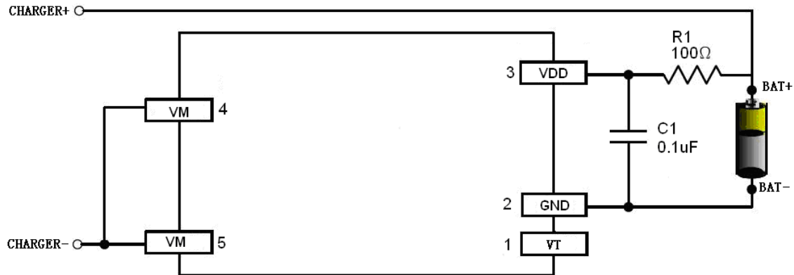
Fig 6 XB5556A0 in a Typical Battery Protection Circuit
