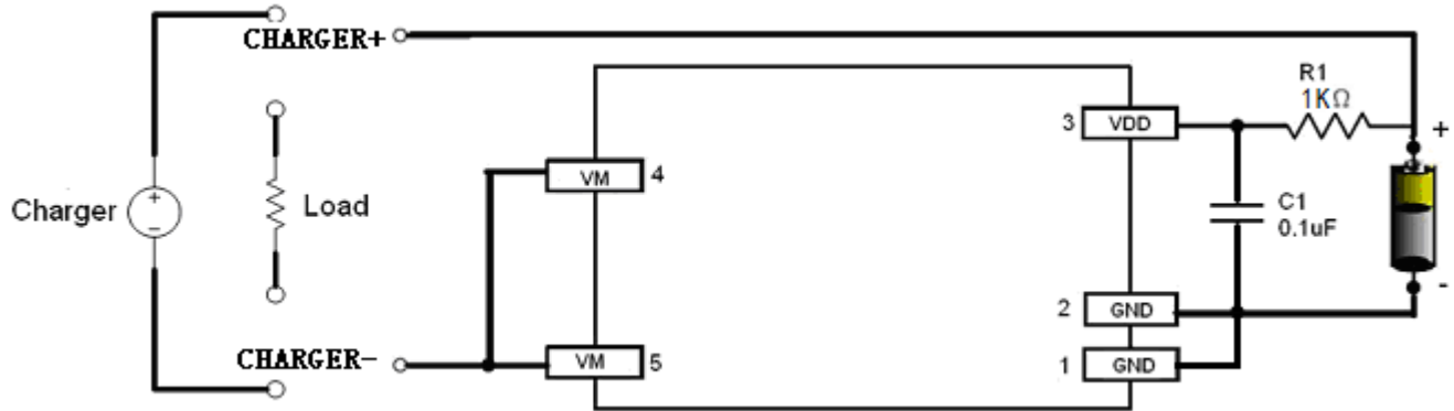
Fig 6 XB5606GJ in a Typical Battery Protection Circuit
