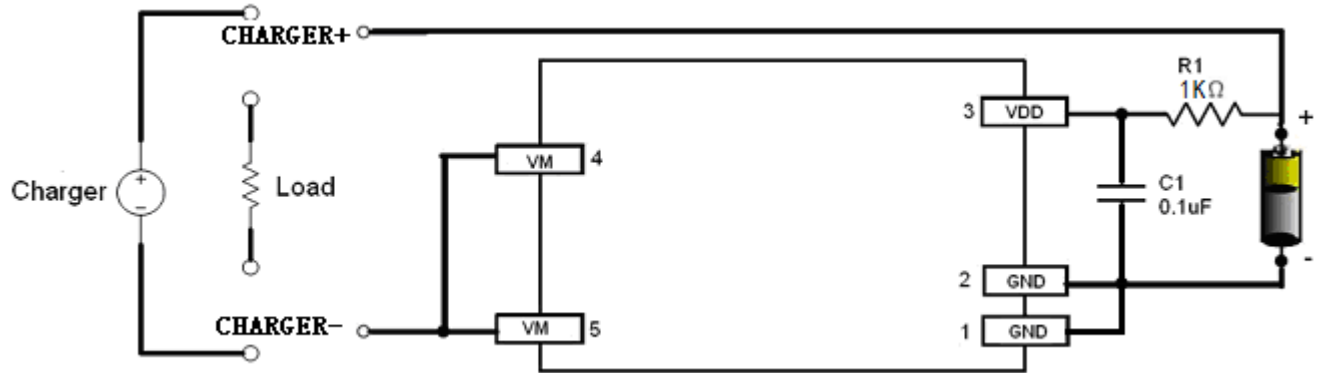
Fig 6 XB5609A in a Typical Battery Protection Circuit
