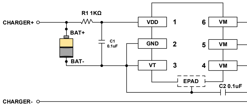
Figure 6 XBG6158 ZR SERIES in a Typical Battery Protection Circuit
