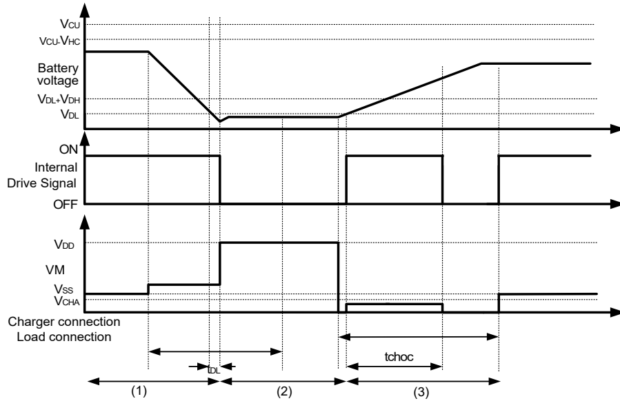
Figure5-3 Abnormal Charger Detection
