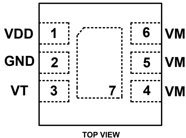
Figure 2. PIN Configuration
