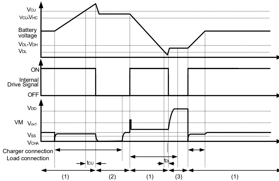
Figure5-1 Overcharge and Overdischarge Voltage Detection
