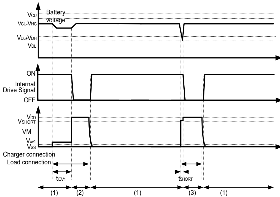
Figure5-2 Overdischarge Current and Short Detection
