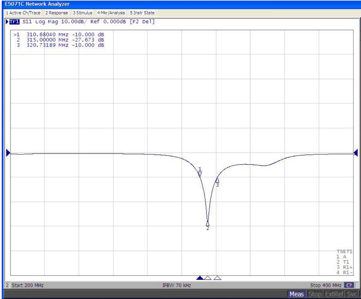
Fig. 4 Return loss
