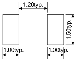
Recommended Pad Layout (mm)
