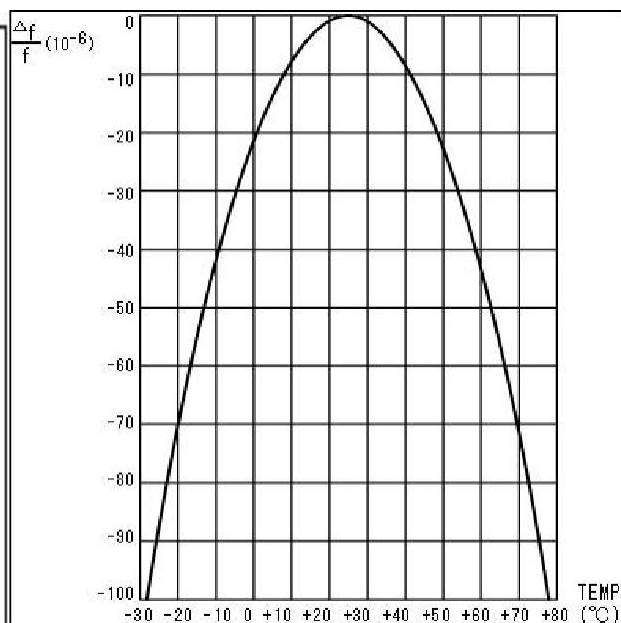
FREQUENCY VS. TEMPERATURE CURVE
