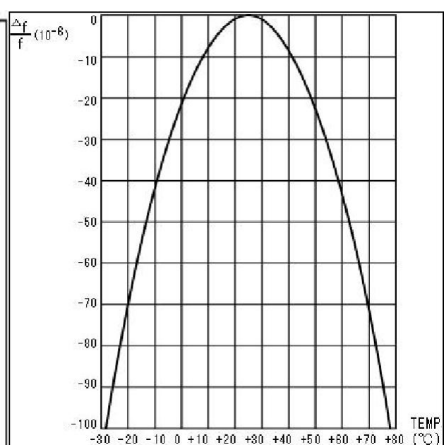
FREQUENCY VS. TEMPERATURE CURVE
