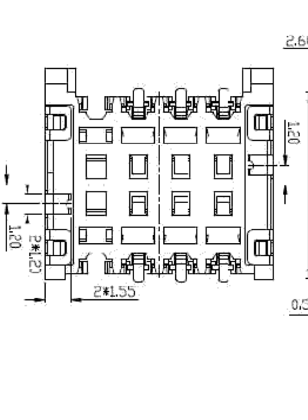
Unit: mm; Tolerances: ±0.15 mm Mechanical outline dimension
