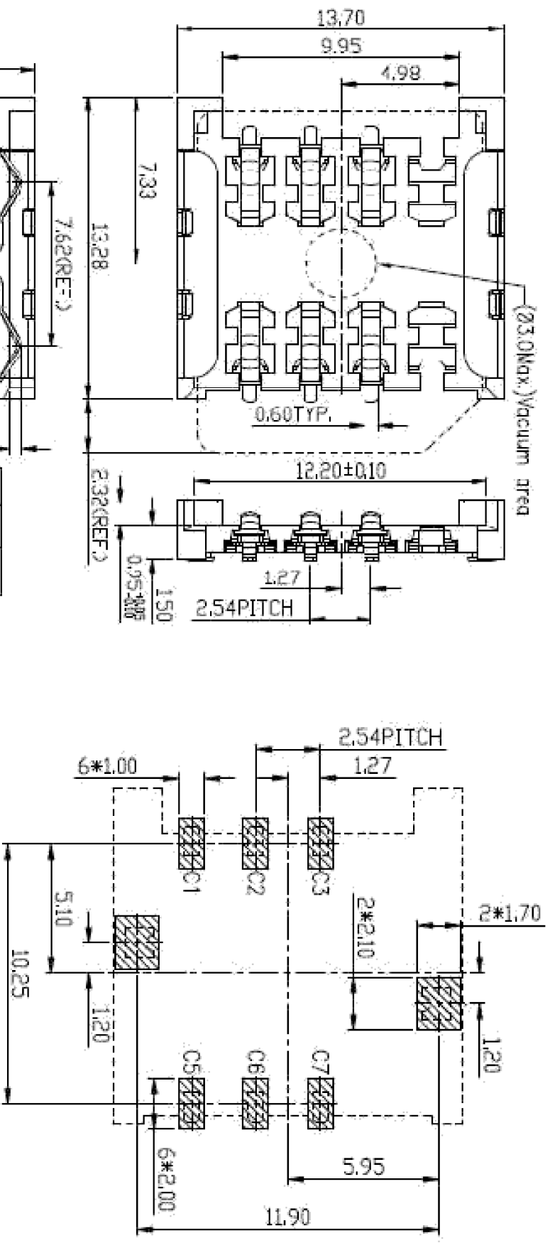
Unit: mm; Tolerances: ±0.05 mm Reference dimension for PCB layout
