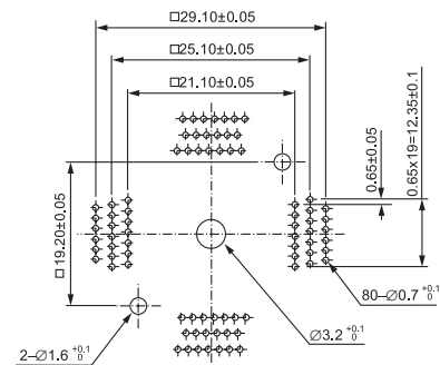
QFP IC201-0804-014 (80 Pins)
