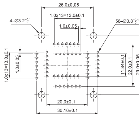
IC51-0564-790 (56 Pins)
