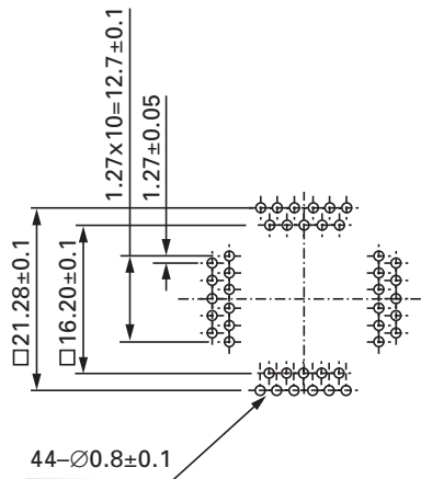
44 pins IC53-0444-306
