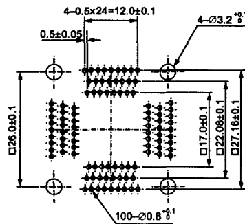
IC51-1004-809 (100 Pins)
