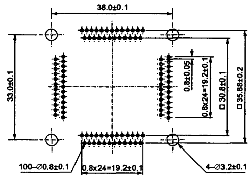
IC51-1124-1036-2 (112 Pins)
