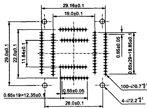
IC51-814-KS12033 (100 Pins)
