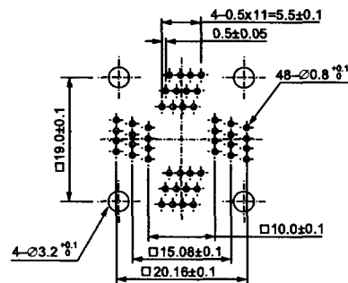
IC51-0484-806 (48 Pins)
