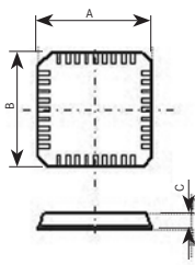
Outline IC Body Dimensions
