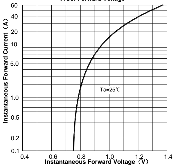
FIG3: Forward Voltage
