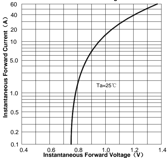
FIG3: Forward Voltage
