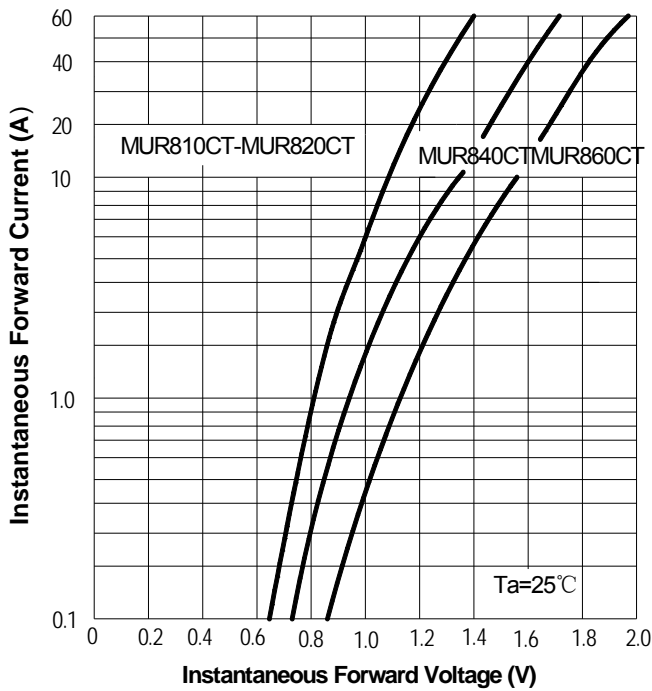
FIG3: Forward Voltage
