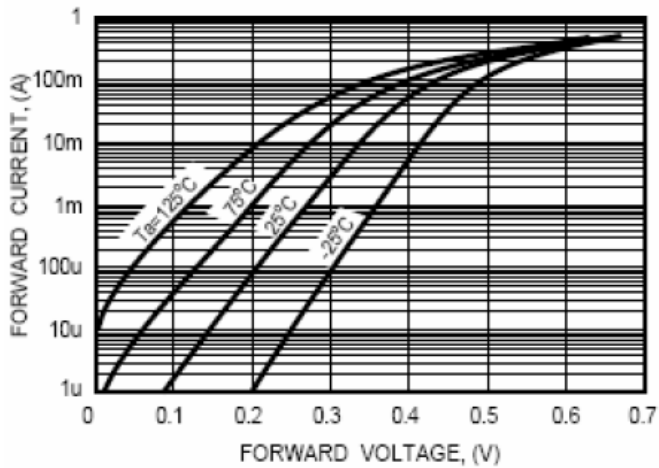
FIG. 1 - FORWARD CHARACTERISTICS
